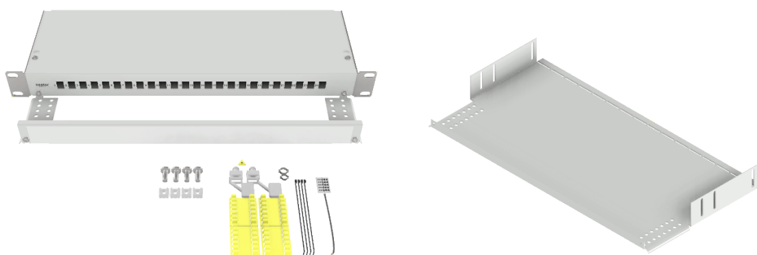
Nestor Panel basic assembly for SC-S adapters (LV2493) and adjustable fiber shelf
