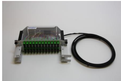
NC-1000 SC/APC 48xSML 50 m
