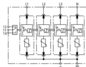
Basic circuit diagram DG M TNS 275 FM
