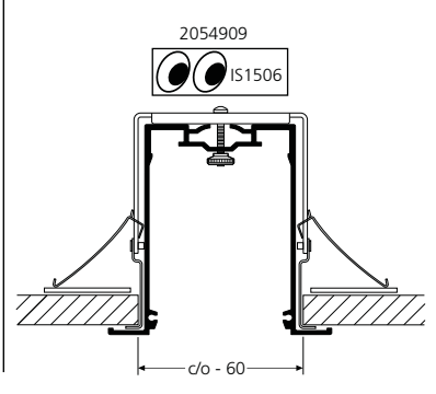
5 +Trim - Recessed
