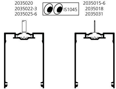
5 Trimless - Suspended
