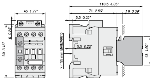
NF..22E, NF..31E, NF..40E + CA4, CC4, 1-napainen apukosketinlohko
