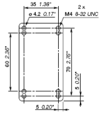
AF09, AF12, AF16
