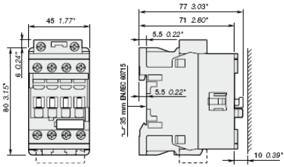
AF09, AF12, AF16
