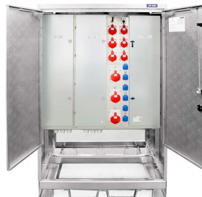
TPK 400C22
